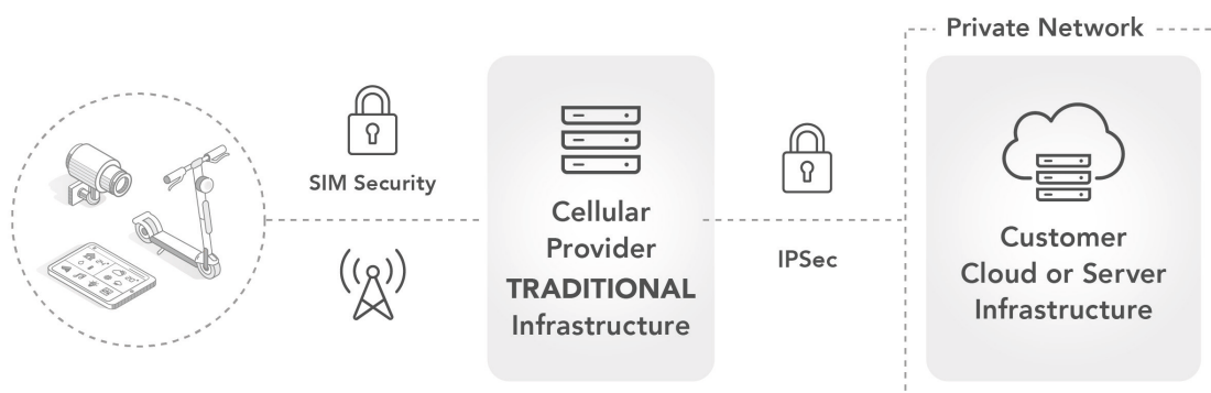
Figure 5 - Network Layer Security between Mobile Network and Infrastructure
